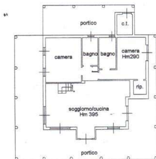
PIANO TERRA
